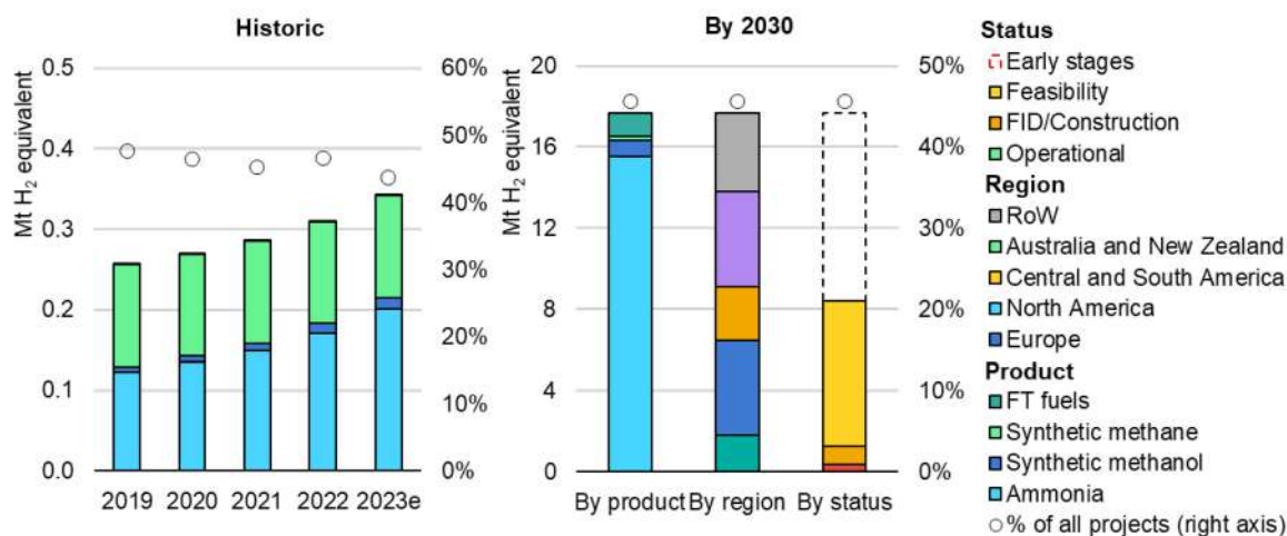
Figure 3.16 Global hydrogen-based fuel production by fuel, region and status, historical and based on announced projects
