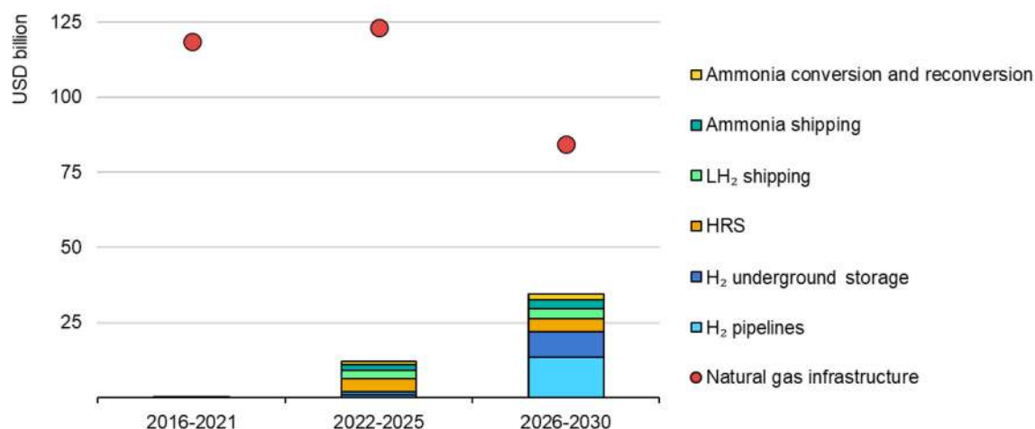
Figure 4.5 Global annual investment in gas infrastructure in the Net Zero Emissions by 2050 Scenario, 2016-2030
