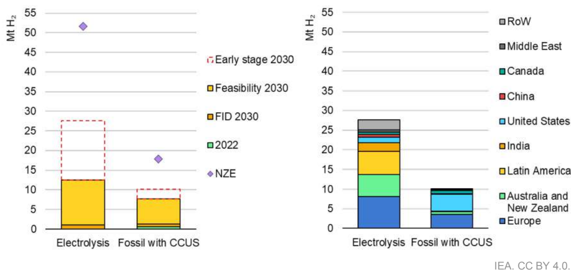
Figure 3.2 Low-emission hydrogen production by technology route, maturity and region based on announced projects and in the Net Zero Emissions by 2050 Scenario, 2030
